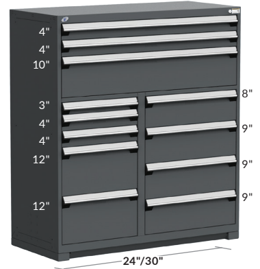
12 DRAWERS R5KJE-5801 54" x 24" x 60" R5KJG-5801 54" x 27" x 60"
