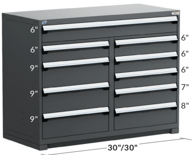
10 DRAWERS R5KKE-4407 60" x 24" x 46" R5KKG-4407 60" x 27" x 46"
