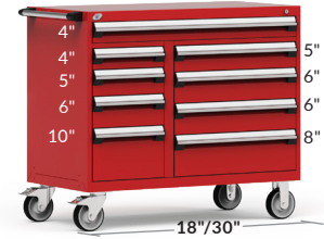
9 DRAWERS R5GHE-3419 48" x 24" x 41 1/2" R5GHG-3419 48" x 27" x 41 1/2"
