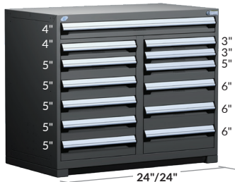
13 DRAWERS R5KHE-3811 48" x 24" x 40" R5KHG-3811 48" x 27" x 40"
