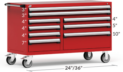
9 DRAWERS R5GKE-3009 60" x 24" x 37½" R5GKG-3009 60" x 27" x 37½"
