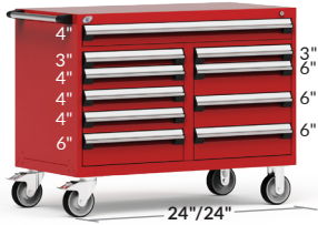
10 DRAWERS R5GHE-3005 48" x 24" x 37 1/2" R5GHG-3005 48" x 27" x 37 1/2"
