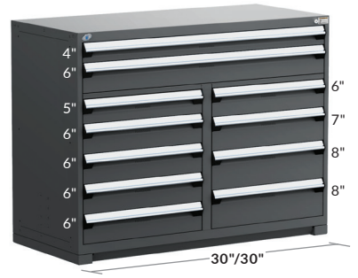
11 DRAWERS R5KKE-4405 60" x 24" x 46" R5KKG-4405 60" x 27" x 46"
