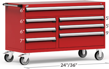
7 DRAWERS R5GKE-3015 60" x 24" x 37½" R5GKG-3015 60" x 27" x 37½"
