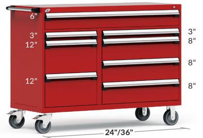
8 DRAWERS R5GKE-3827 60" x 24" x 45½" R5GKG-3827 60" x 27" x 45½"
