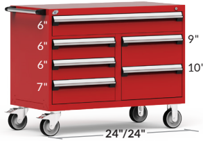
6 DRAWERS R5GHE-3019 48" x 24" x 37 1/2" R5GHG-3019 48" x 27" x 37 1/2"
