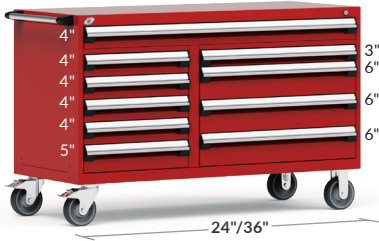
10 DRAWERS R5GKE-3005 60" x 24" x 37½" R5GKG-3005 60" x 27" x 37½"
