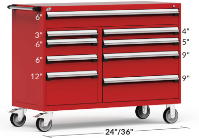
9 DRAWERS R5GKE-3823 60" x 24" x 45½" R5GKG-3823 60" x 27" x 45½"
