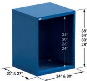
24" and 30" Wide
